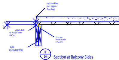
Section at Balcony Sides
