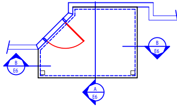
ENLARGED "A2" TYPE BALCONY
