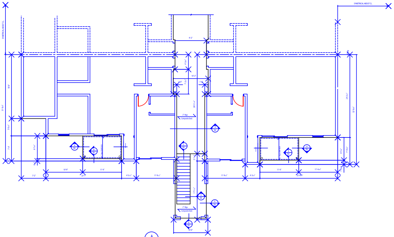
A E4 BLDG. "B" ENLARGED AREA PLAN
