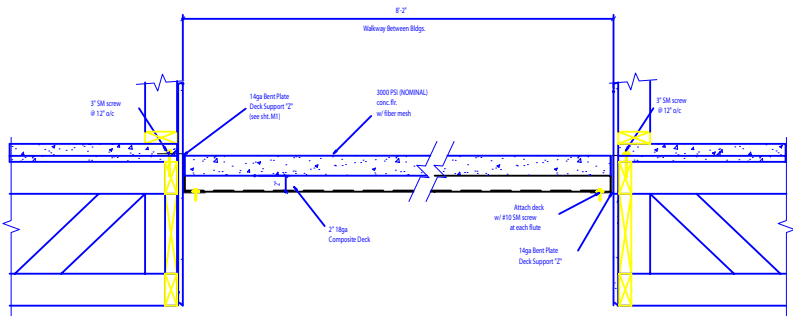
D E6 Section Thru Breezeway
